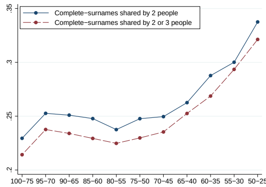
Figure 11: Evolution of Sibling Correlation Proxy, SCP over moving windows of cohorts.
