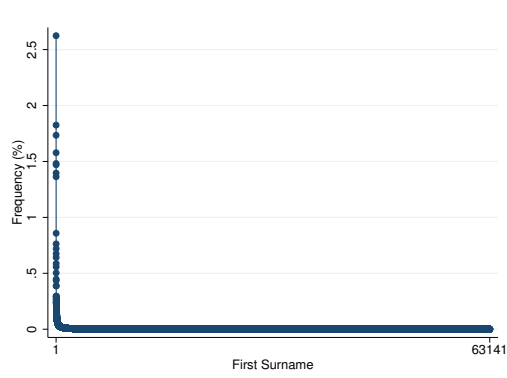
(a) Distribution of First Surname
