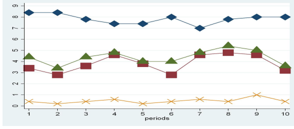
(a) Effort-Majority (1.1)
