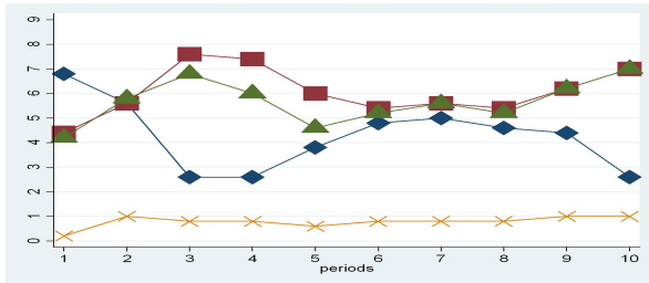
(i) Effort-Majority (5.1)
