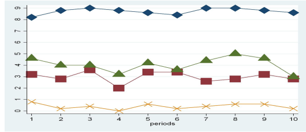
(f) Effort-Exclusion (3.2)
