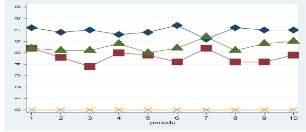
(b) Unanimity (1.2)
