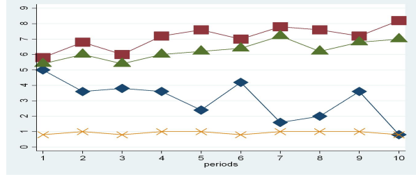
(b) Effort-Majority (1.2)
