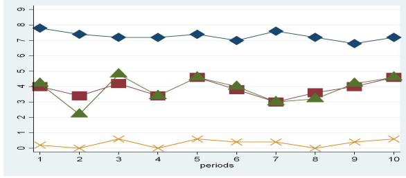
(c) Effort-Majority (2.1)
