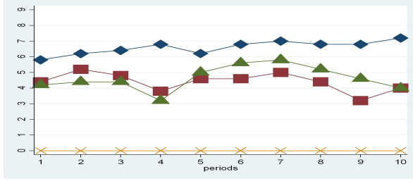
(a) Unanimity(1.1)
