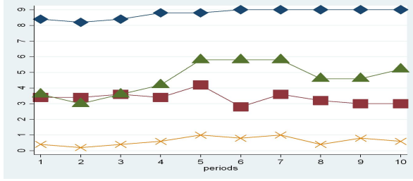
(a) Effort-Exclusion(1.1)
