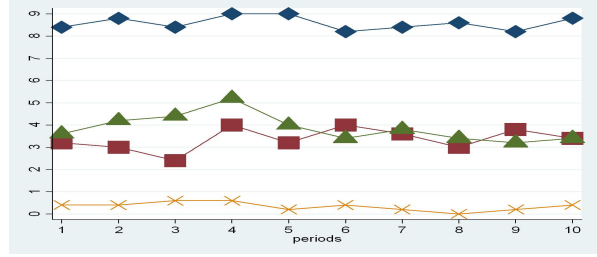
(b) Effort-Exclusion (1.2)
