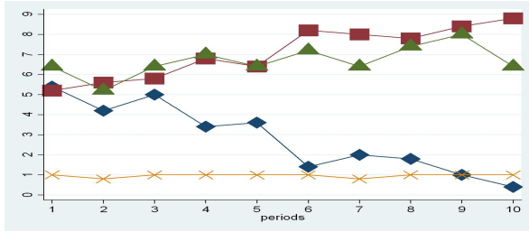
(g) Effort-Majority (4.1)
