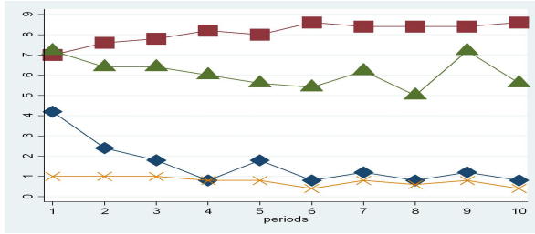
(e) Effort-Majority (3.1)
